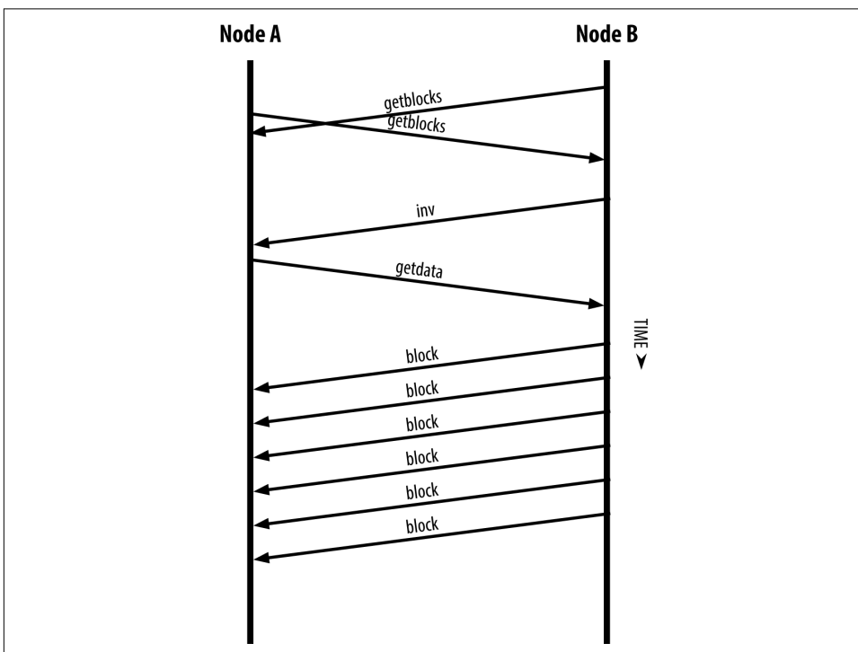
Figure 8-6. Node synchronizing the blockchain by retrieving blocks from a peer
