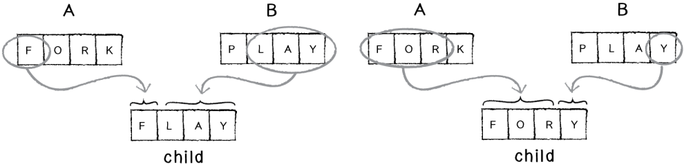
Figure 9.4: Picking a random midpoint
